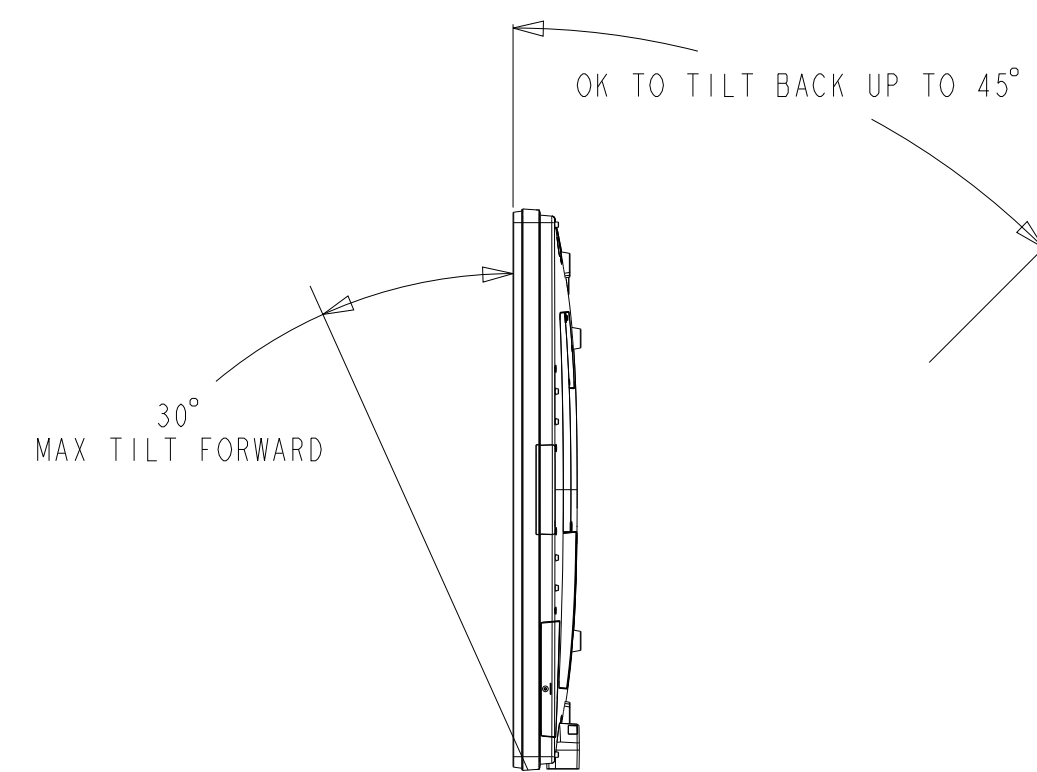
TILTING REQUIREMENTS
