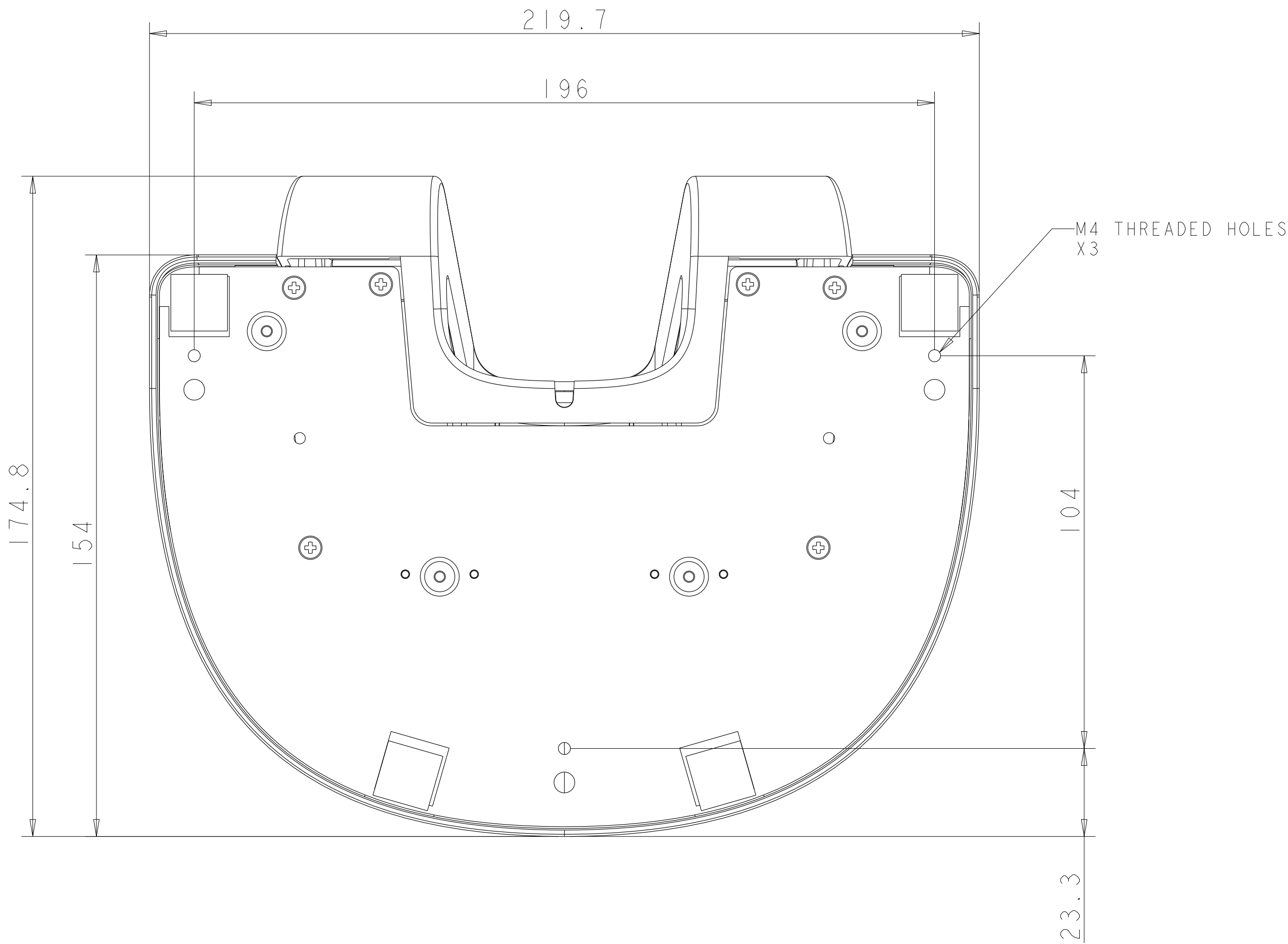
BOTTOM VIEW
