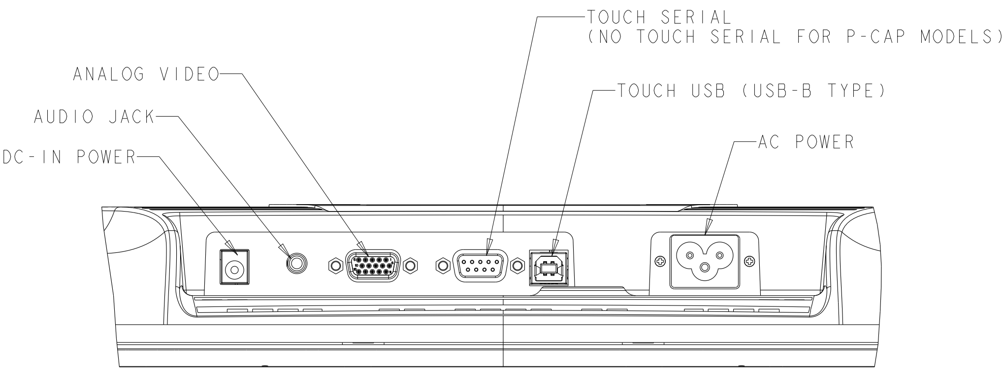
ET1515L WITH SPEAKER AND DC POWER (CUSTOMIZED)
