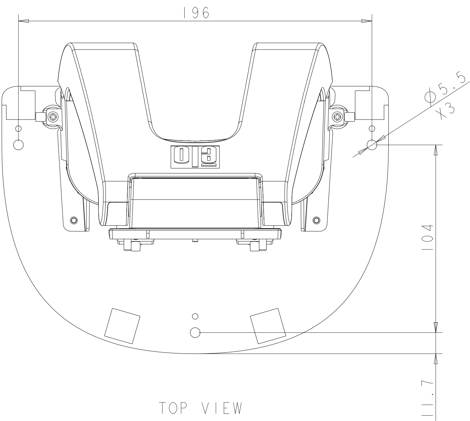
MOUNT OPTION 1
