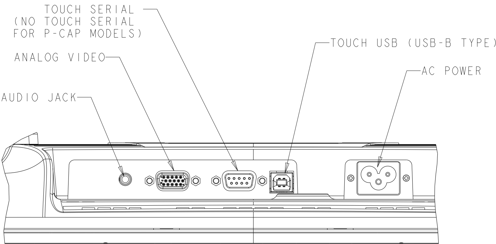
ET1515L WITH SPEAKER (CUSTOMIZED)
