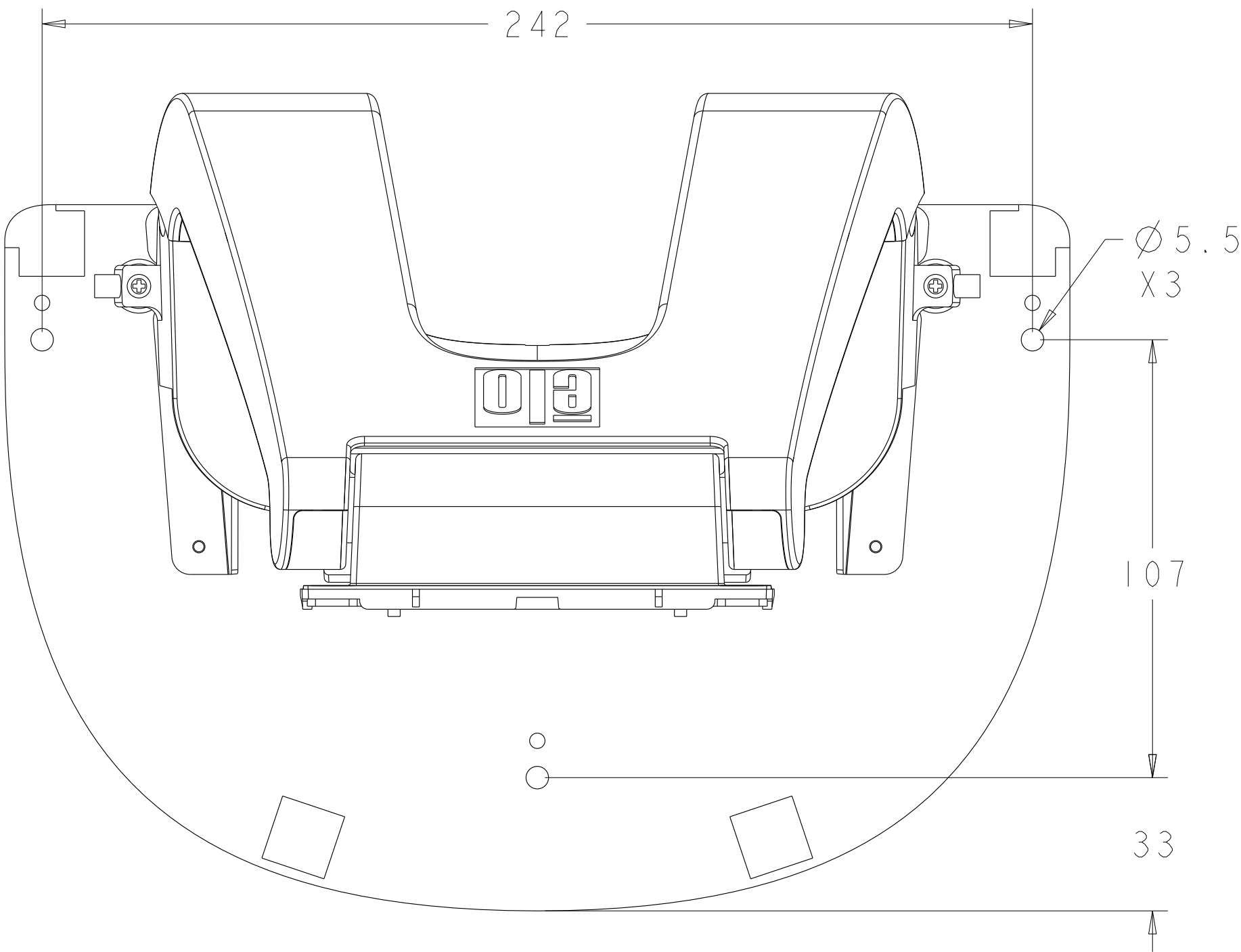
TOP VIEW
