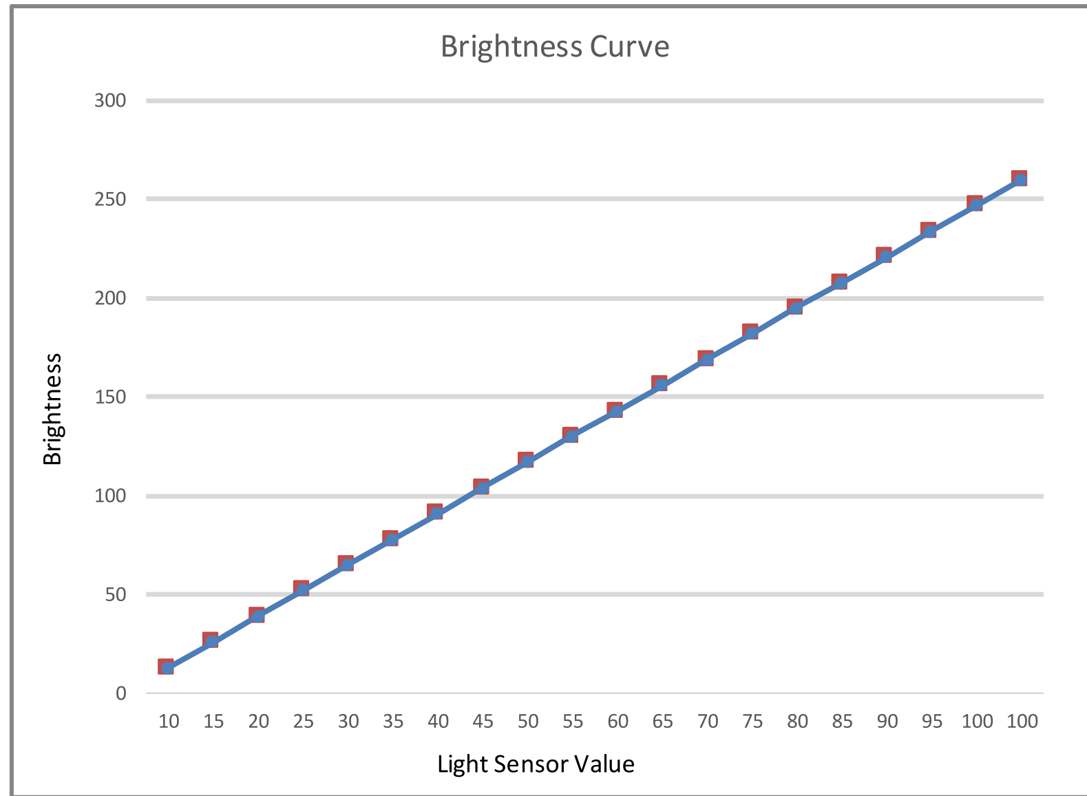
Light Sensor Curve
