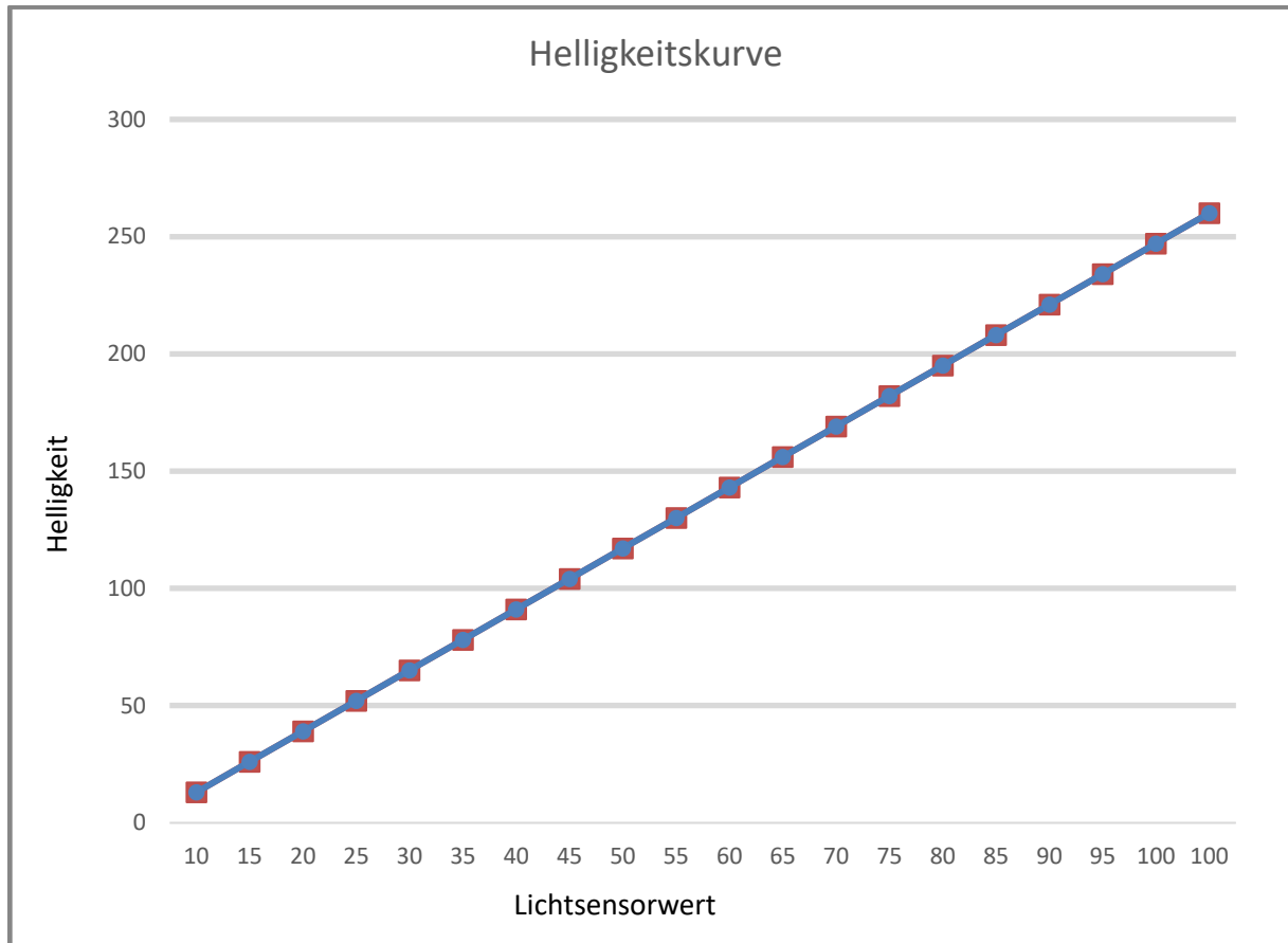
Lichtsensorcurve
