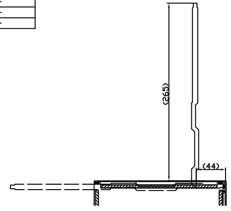
FPC folding shape
