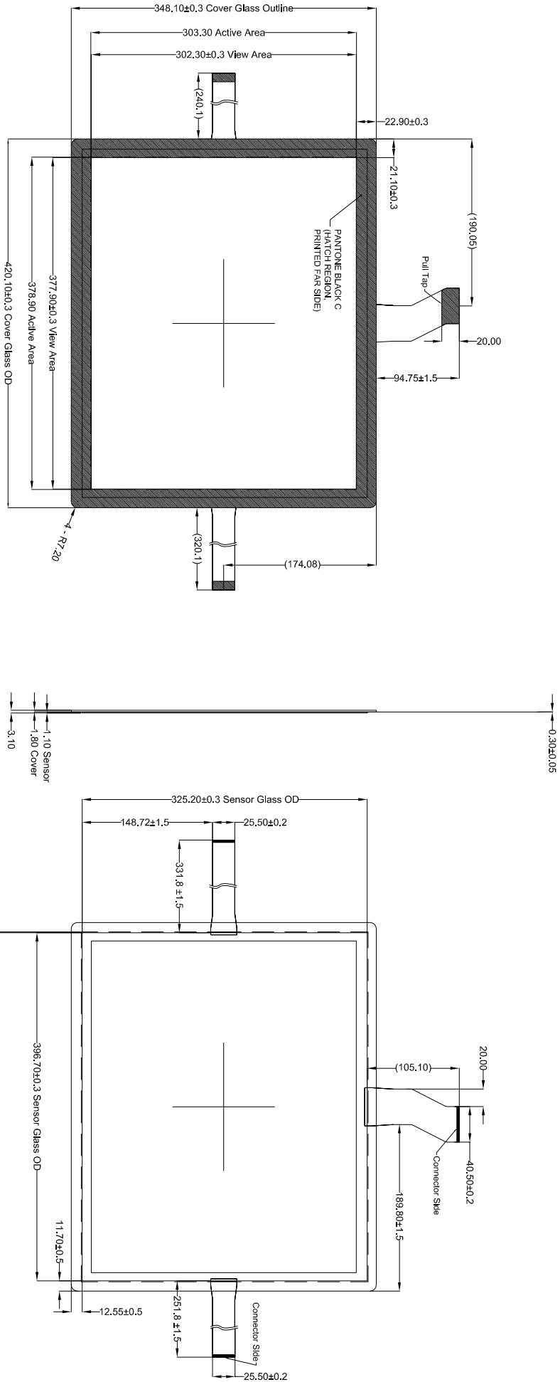
Front View
