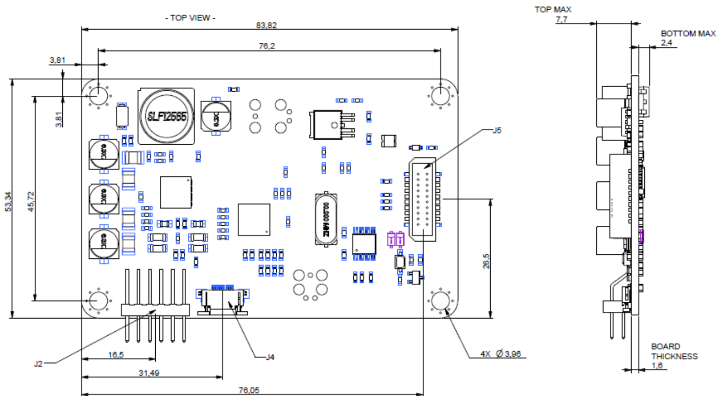
Figure 2.6 CTR-3200 dimensions (CTR-320004-IT-RSU-001-R)
