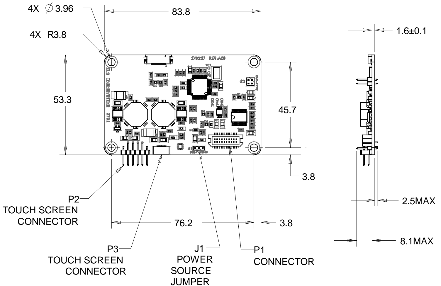
Figure 2-7. 2701 Dimensions: Top and Side Views (CTR-270100-IT-RSU-00R)
