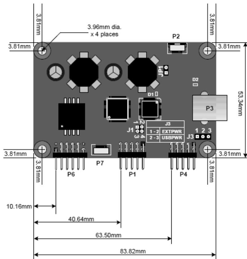
Figure 2-8. 2515 Dimensions (CTR-251500-IT-USB-07-R)
