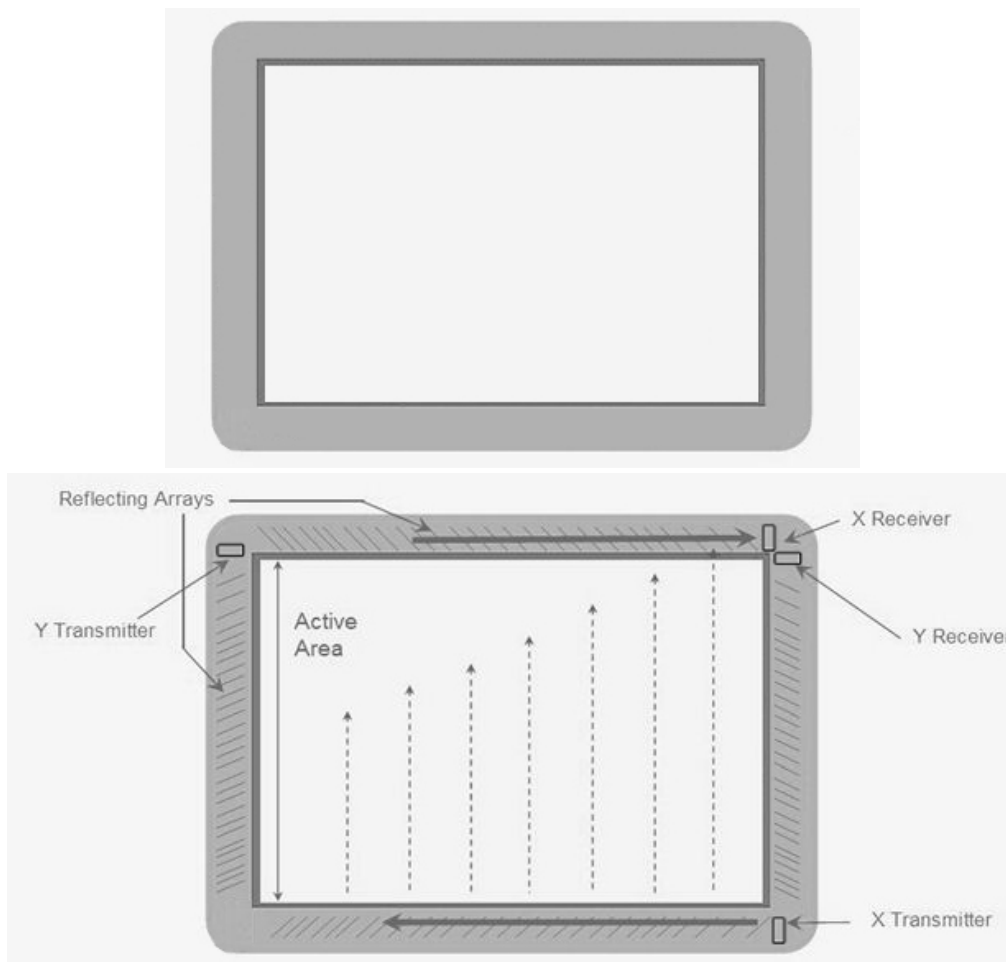
Figure 1-1. Front and Back of IntelliTouch® ZB Touchscreen
