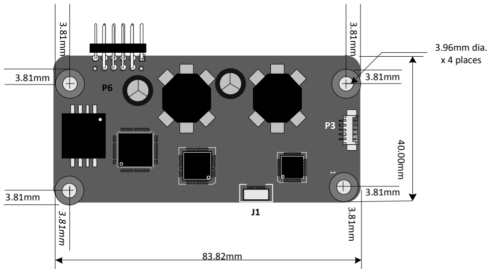
Figure 2-9. 2520 Dimensions (CTR-252000-IT-USB-00-R)
