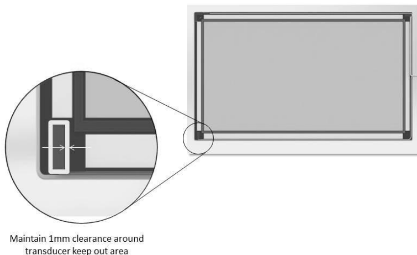
Figure 2-3. Clearance gap around transducers
