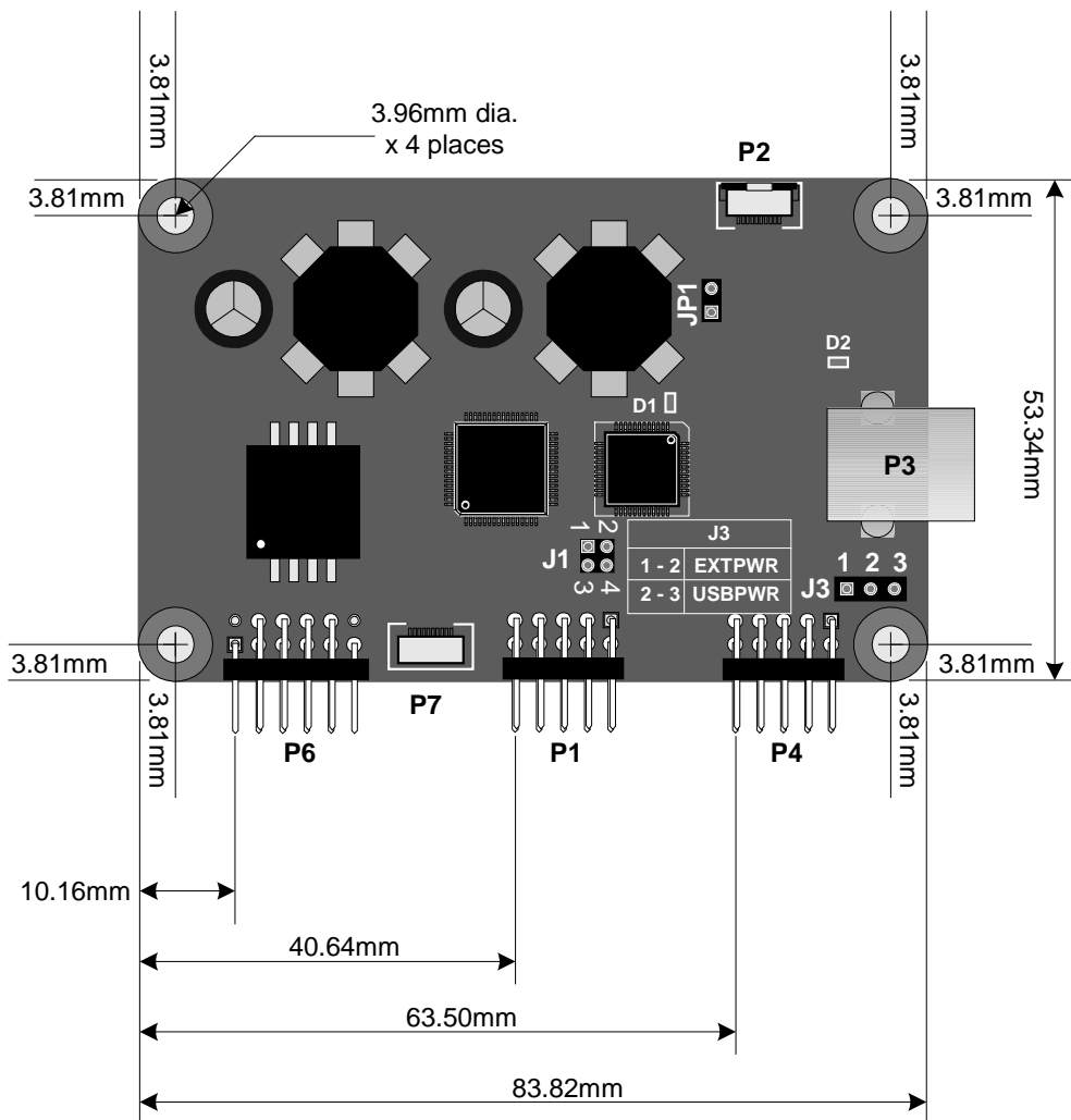
Figure 2-10. 2521 Dimensions (CTR-252100-IT-USB-00-R)
