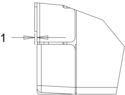
DETAIL A CENTERING LIP, TYPICAL SCALE 2.000
