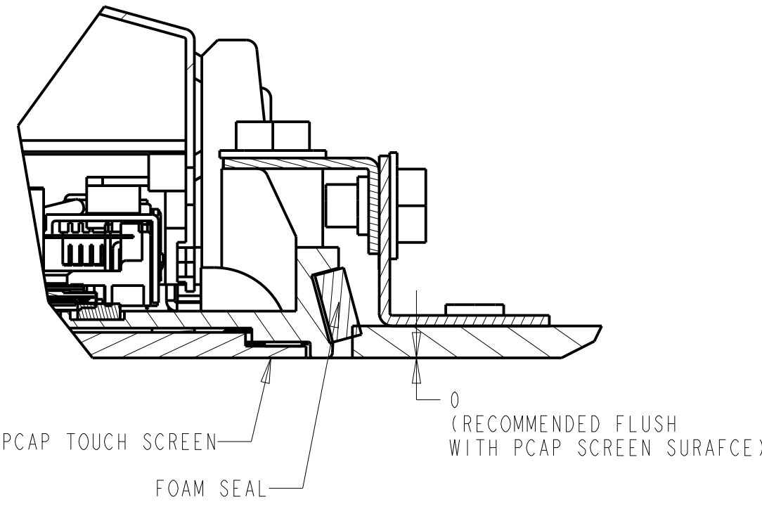
SECTION A-A SCALE 1:500
